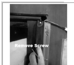
Figure 8 Removing the bulb seal screw
