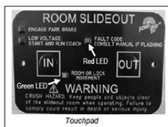
Fig.1 Slideout Controller
